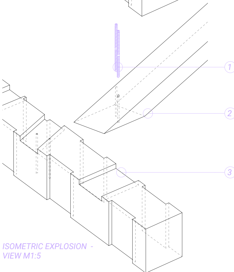
ISOMETRIC VIEW M1:5
