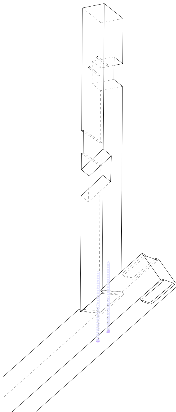
ISOMETRIC EXPLOSION - VIEW M1:5
