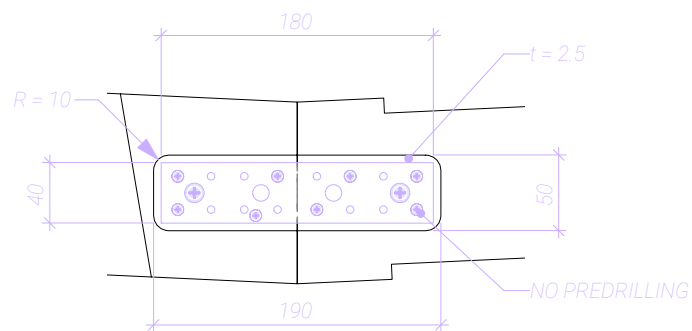
TOP VIEW M1:5
