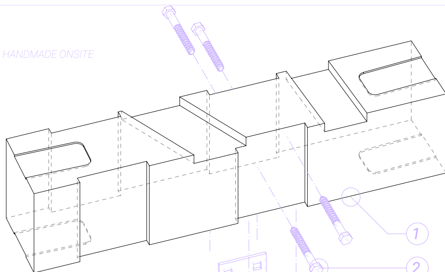
ISOMETRIC EXPLOSION - VIEW M1:5
