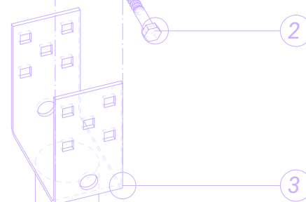
ISOMETRIC EXPLOSION - VIEW M1:5
