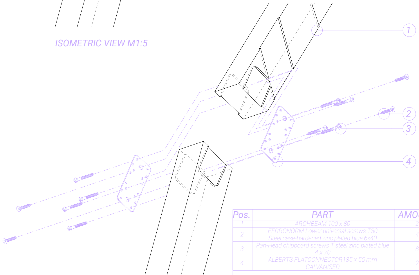
ISOMETRIC EXPLOSION - VIEW M1:5
